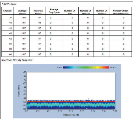
Figure 8: Intergrated reporting
